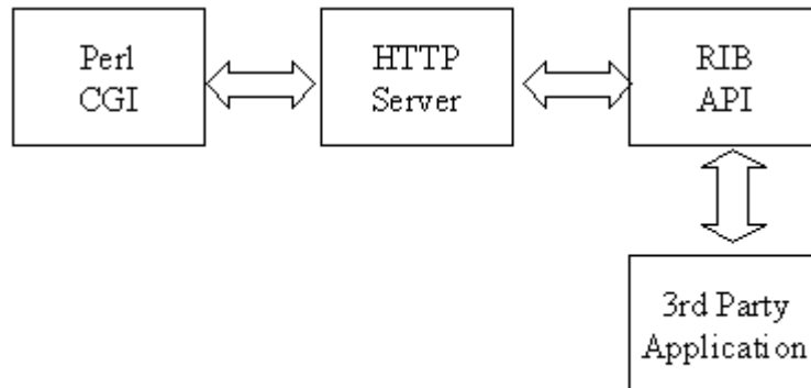
Figure 2. RIBAPI Dataflow
