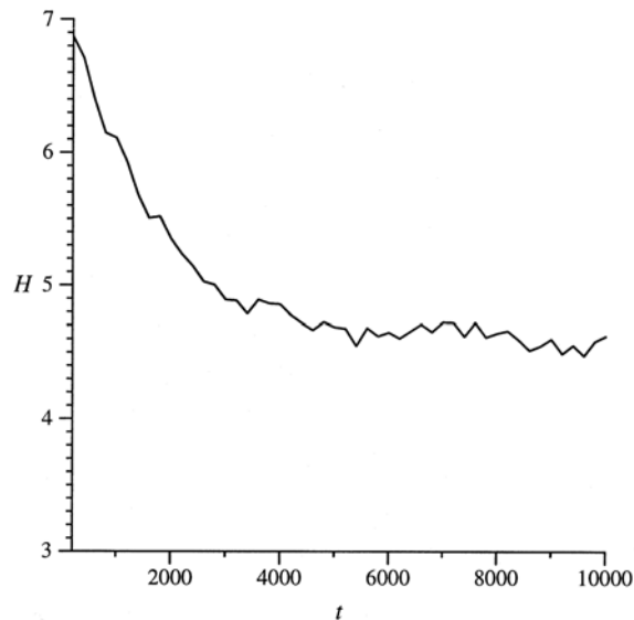
Figure 6: Entropy: Two-symbol Communication.
