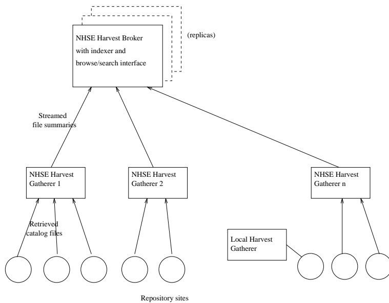
Figure 2: Indexing using Harvest
