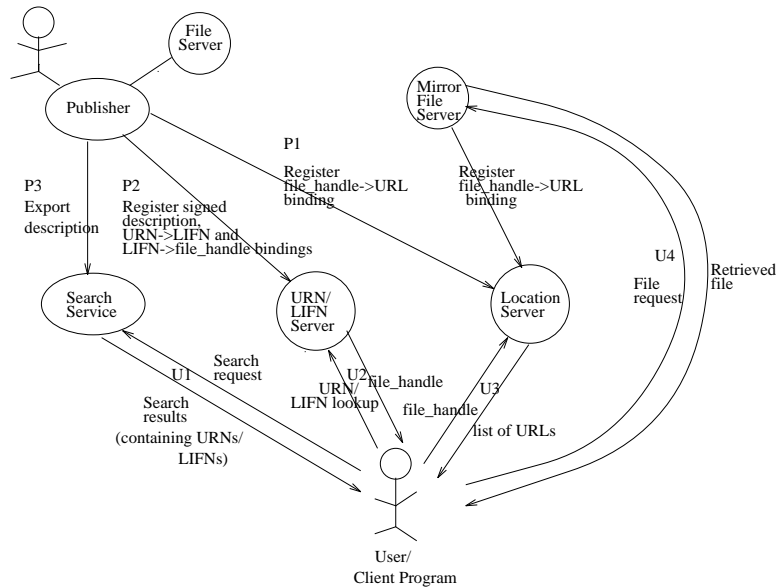
Figure 3: Publishing and Retrieving Assets Using Location-Independent Naming
