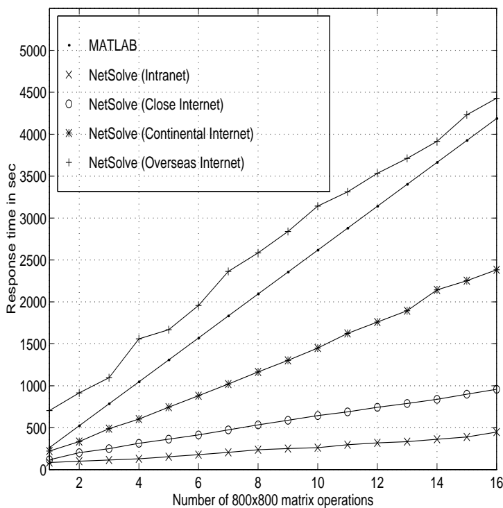
Figure 2: Multiple 400x400 matrix multiplications
