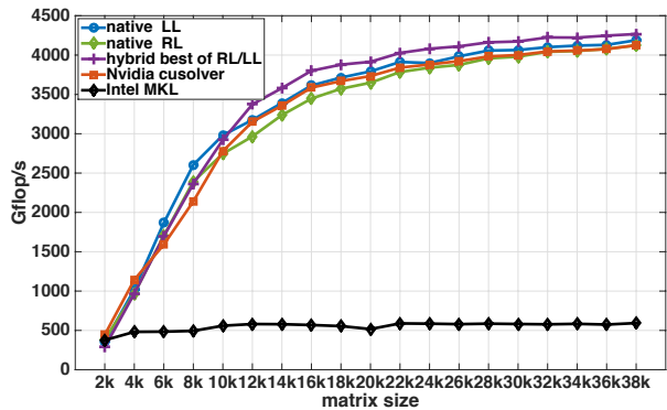
Figure 17: Performance comparison of the native GPU-only, hybrid CPU-GPU and CPU-only Cholesky factorization on the Nvidia P100 GPU using double precision dpotrf routine.
