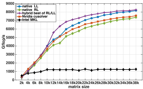
Figure 16: Performance comparison of the native GPU-only, hybrid CPU-GPU and CPU-only Cholesky factorization on the Nvidia P100 GPU using single precision spotrf routine.
