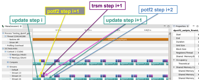
Figure 13: Nvidia profiler snapshot showing the lookahead potf2 computation executed on stream 15 overlapped with the update phase running on stream 16 for the left looking native variant.
