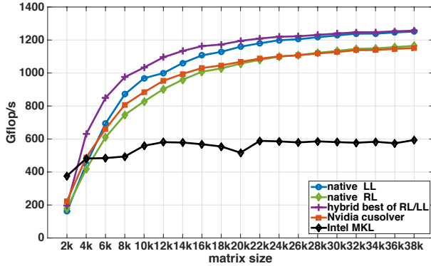
Figure 15: Performance comparison of the native GPU-only, hybrid CPU-GPU and CPU-only Cholesky factorization on the Nvidia K40c GPU using double precision dpotrf routine.
