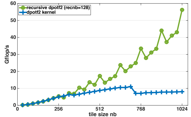
Figure 10: Effect of the recursive design of the dpotf2 routine on a Nvidia P100 GPU.
