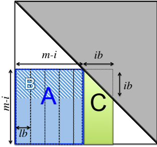
Figure 8: left-looking Cholesky factorization
