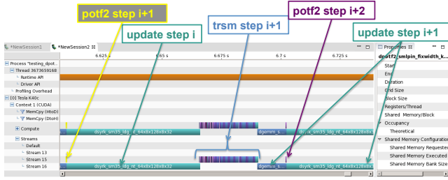
Figure 12: Nvidia profiler snapshot showing the lookahead potf2 computation executed on stream 15 overlapped with the update phase running on stream 16 for the right looking native variant.
