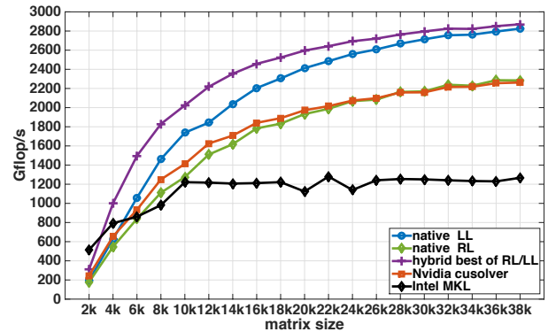
Figure 14: Performance comparison of the native GPU-only, hybrid CPU-GPU and CPU-only Cholesky factorization on the Nvidia K40c GPU using single precision spotrf routine.
