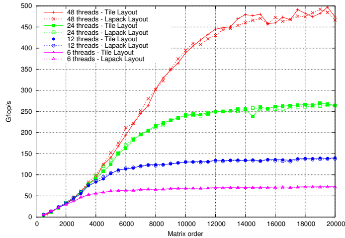
Fig. 11. Scalability of PLASMA recursive LU on MagnyCour-48 in single precision.
