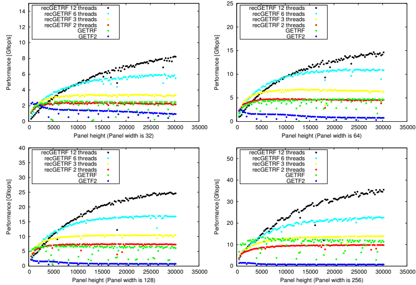
Fig. 6. Scalability study of the recursive parallel panel factorization in double precision on tile layout with various panel widths: 32 (top-left), 64 (top-right), 128 (bottom-left), and 256 (bottom-right).
