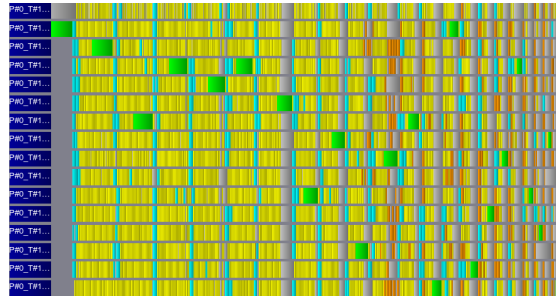
(b) Recursive LU DGETRF with sequential panel factorization, N = 5000 and NB = 220
