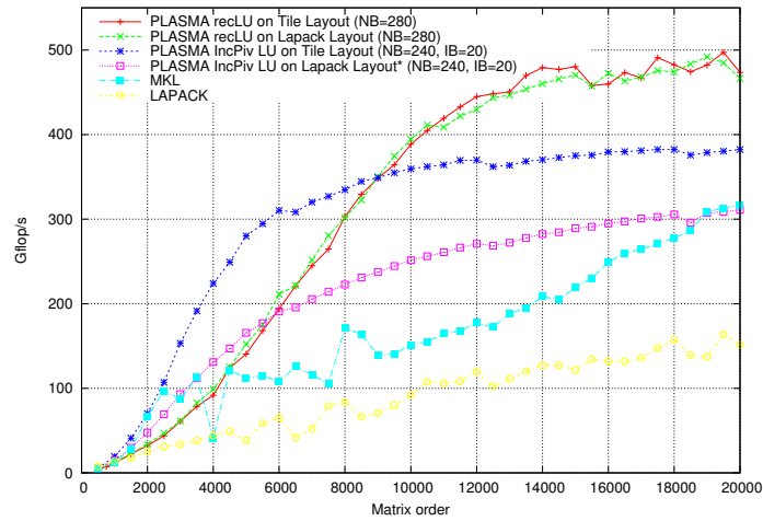
Fig. 9. Performances of SGETRF on MagnyCour-48 .
