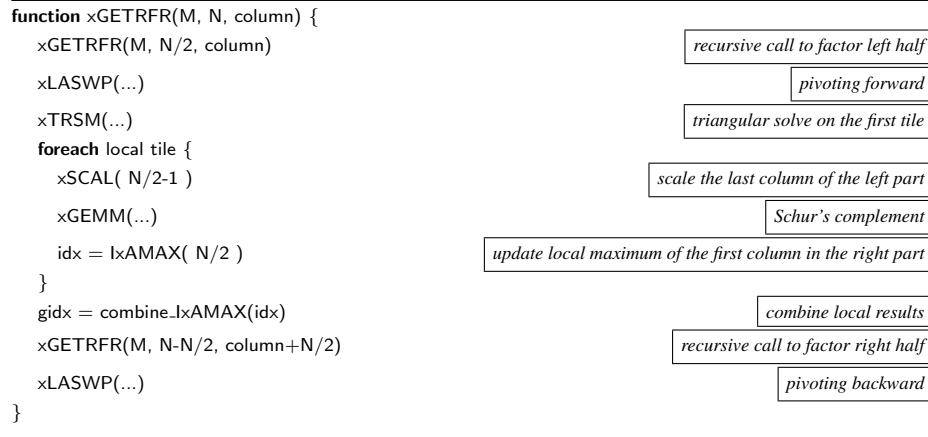
Fig. 4. Pseudo-code for the recursive panel factorization on tile layout.
