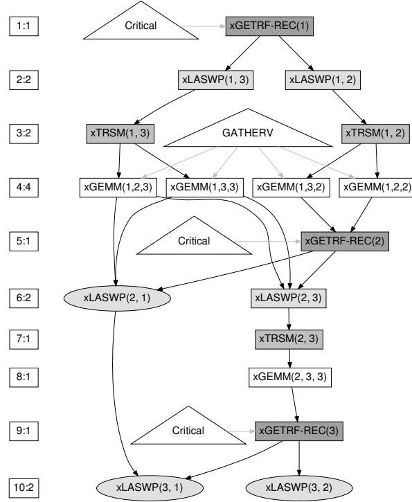
Fig. 8. Annotated DAG for parallel recursive tile LU factorization of a 3-by-3 tile matrix. The annotations are indicated with triangles.
