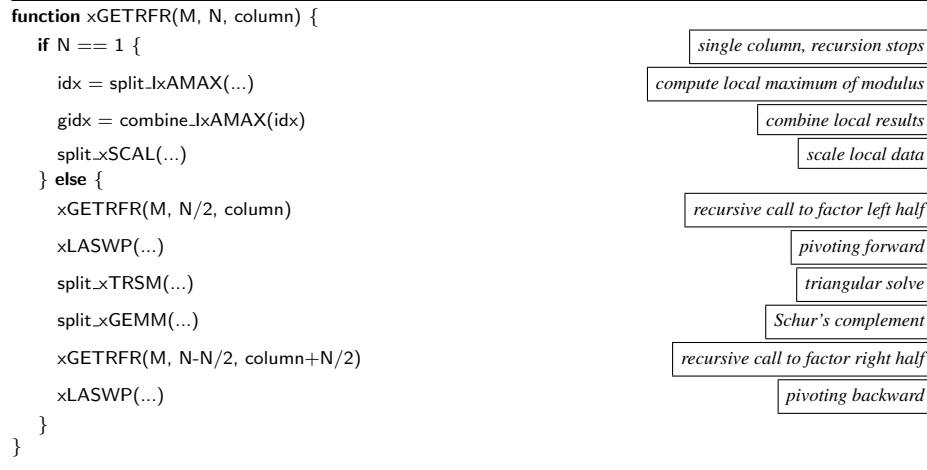
Fig. 2. Pseudo-code for the recursive panel factorization on column major layout.
