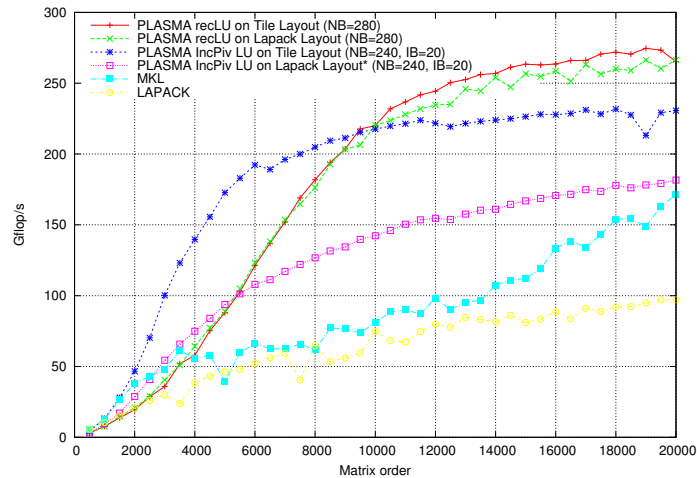
Fig. 10. Performances of DGETRF on MagnyCour-48 .
