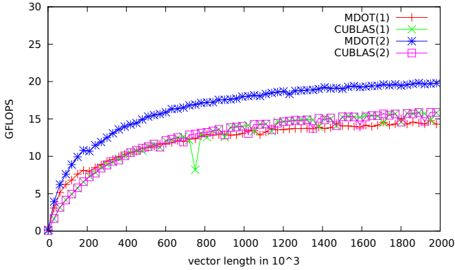
Fig. 8. Performance comparison (double precision) between CUBLAS and MDOT executing 1 and 2 vector products.
