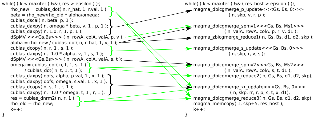
Fig. 3. Visualizing the reformulation of the BiCGSTAB implementation. While all parameters remain in GPU memory, note the explicit transfer of the residual back to the host in the last line.
