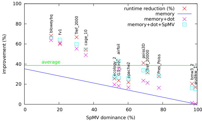
Fig. 11. Performance improvement by replacing the CUBLAS reference implementation with the reformulated version depending on the matrix vector kernel dominance in the original code.
