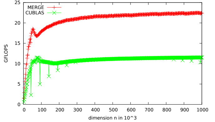
Fig. 5. Performance comparison between the merged BiCGSTAB and the reference implementation for the update of vector p (see line 11 of Figure 1).
