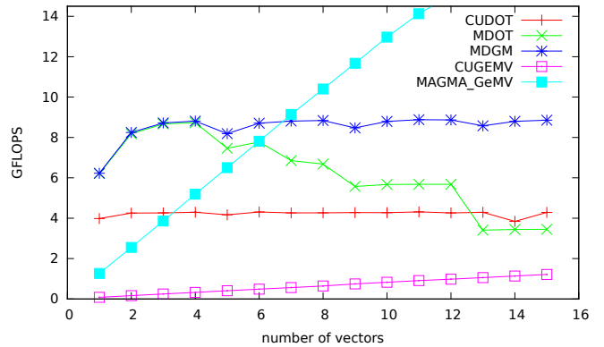
Fig. 6. Performance comparison between CUBLAS dot product, the developed simultaneous dot product implementations MDOT and MDGM, and the matrix vector products from NVIDIA and MAGMA, respectively for a vector length of 100,000.
