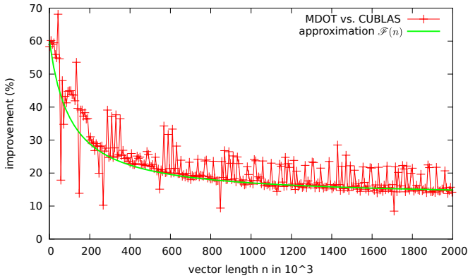
Fig. 10. Size-dependent runtime improvement obtained by replacing CUBLAS with MDOT in the sequence of dot products in BiCGSTAB.
