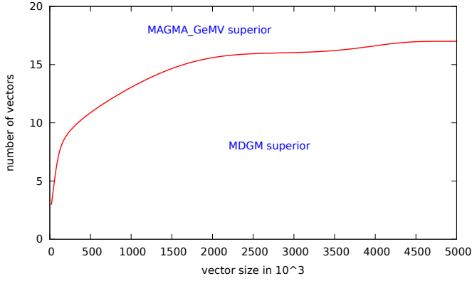
Fig. 7. Superiority areas of MDGM and MAGMA's matrix vector kernel.
