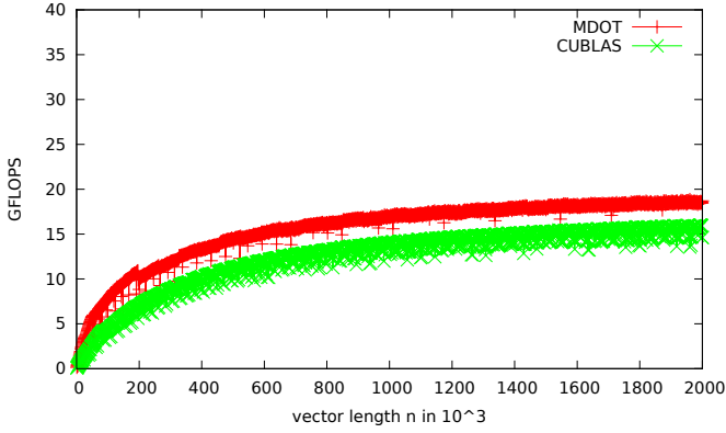
Fig. 9. Performance comparison between CUBLAS and MDOT for the sequence of dot products in one BiCGSTAB iteration.
